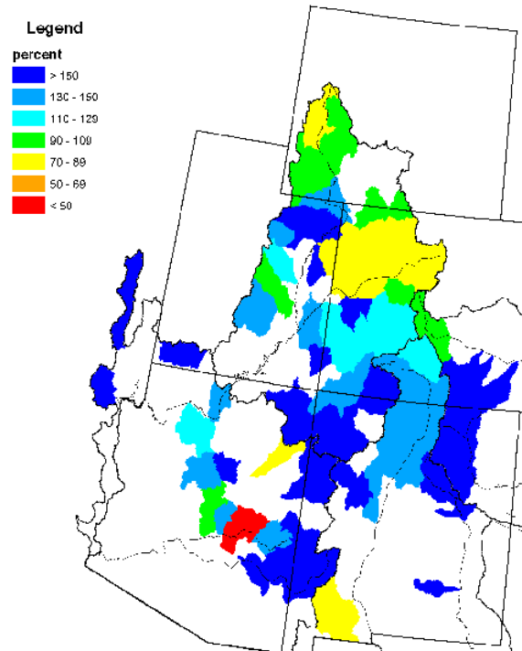
Mountain Snowpack as of April 1, 2005
